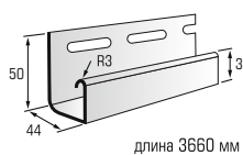
4 J-trim
